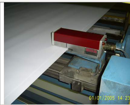
Model 1032 Classic® Splice Detector™ Jagenberg
