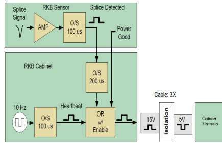
Figure 1: RKB System Block Diagram
