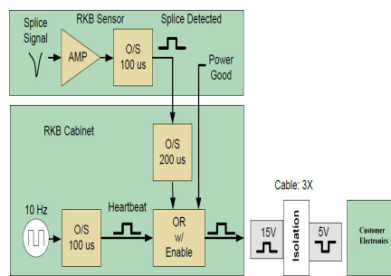
Figure 1: RKB System Block Diagram
