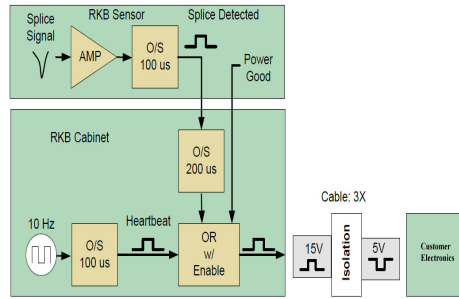
Figure 1: RKB System Block Diagram
